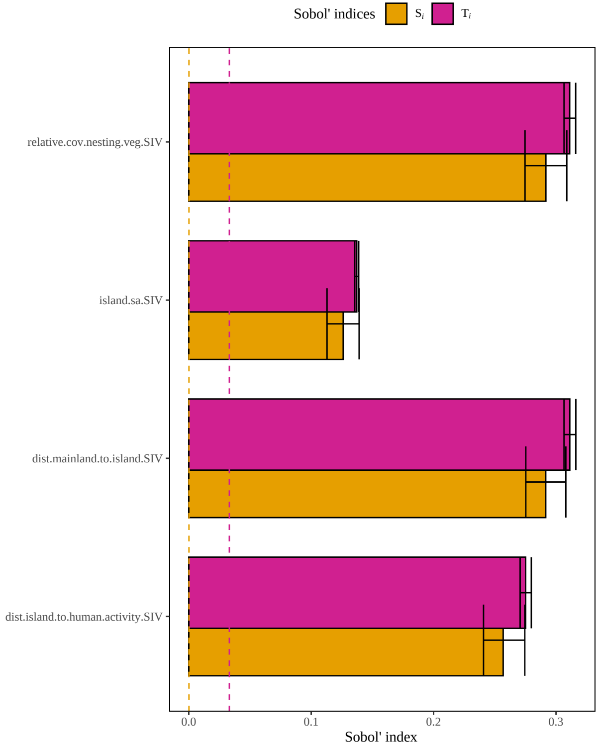
Figure 5. Results of a sensitivity analysis for the easternbrownpelican model based on a geometric mean structure. Dashed lines represent baseline numerical approximation error for S_i and T_i ( i.e. , dummy variables).
